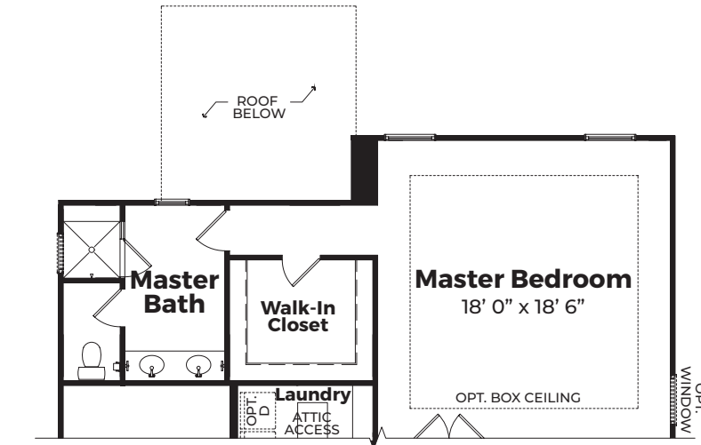
Optional 4' Extension on Owner's Suite
